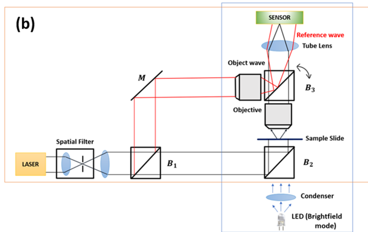
Figure 1. Digital holographic microscope system used in the present study. (a) System photograph. (b) Nominal optical layout of the system. B_1, B_2, B_3 : beam-splitters; M : plane mirror. The beam-splitter B_3 can be rotated with an adjustable screw in order to introduce tilt in the reference wave as required for off-axis hologram recording. The system is fitted with a laser source for phase imaging and LED illumination with condenser for bright-field illumination. By switching between the two illuminations, one can record an image plane digital hologram or a bright-field image of the sample in the same position.
